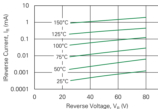
Typical Reverse Current vs. Reverse Voltage
