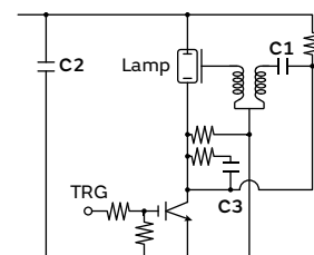
◆Boost current control circuit
