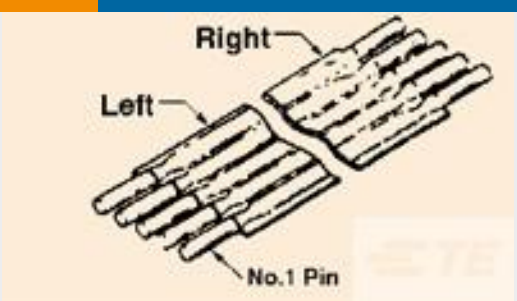
TE Part #9-1447182-8 FSN-11.5A-25=JUMPER NOMEX
