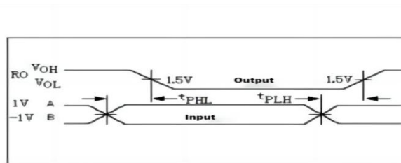
Figure 7: Receiver propagation delay
