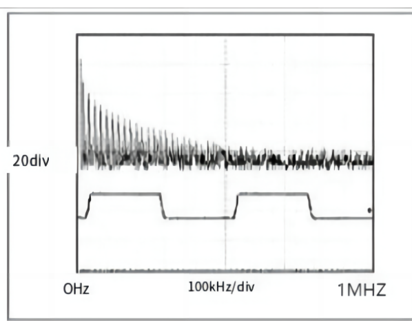
Figure 9: SP490 driver when transmitting 20kHz signal
