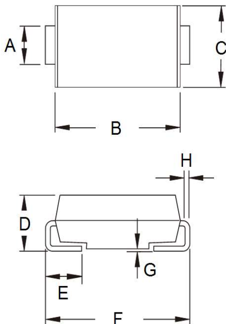
DO-214AA (SMB)
