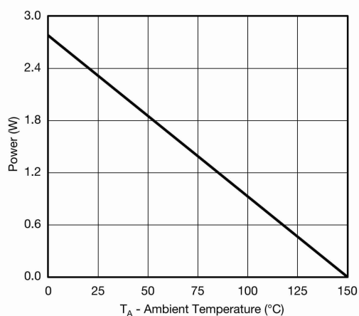
Power, Junction-to-Ambient
