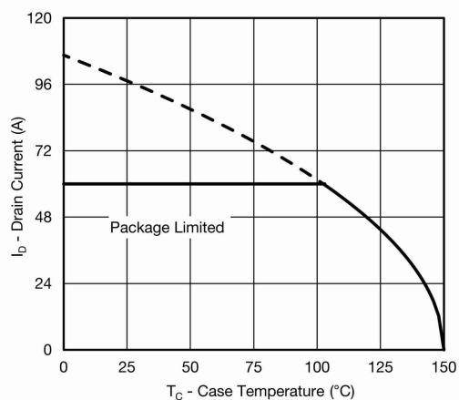
Current Derating*
