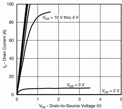
Output Characteristics
