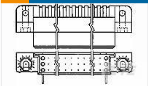
TE Part #532431-8 HDI RECP ASSY 3 ROW 165 POS
