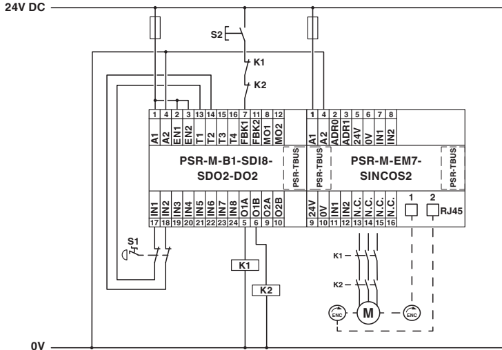
Application drawing
