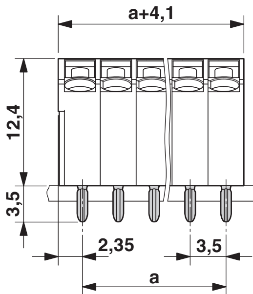
Dimensional drawing
