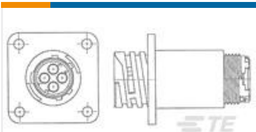
TE Part #796286-1 RCPT.ASSY,23-37STD SEX SQ.FLNG
