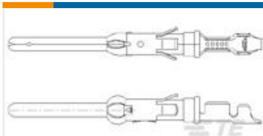
TE Part #163086-1 062 PIN ASS. TYP3+
