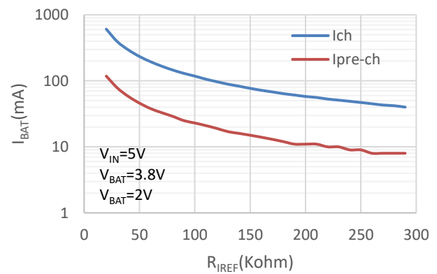
I_{BAT} vs R_{IREF}
