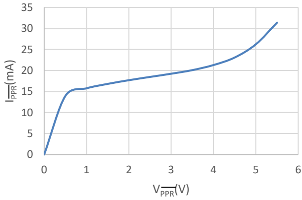
\overline{I_{PPR}} vs \overline{V_{PPR}}
