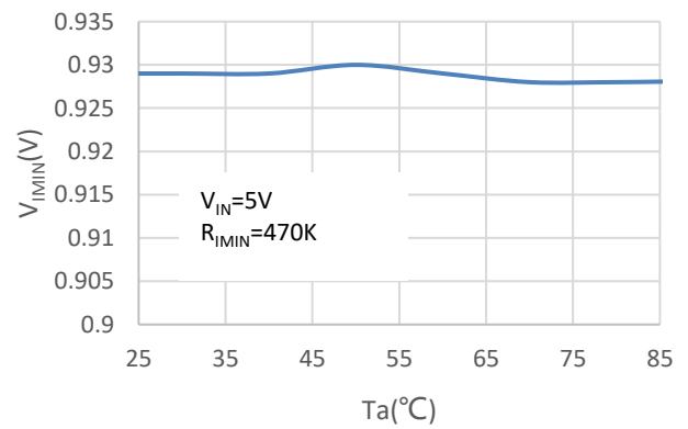
V_{IMIN} vs T_a
