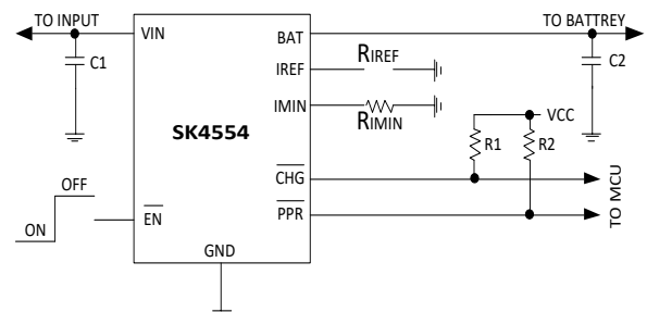
Figure 2. Typical application circuit with the indication signals interfacing to an MCU
