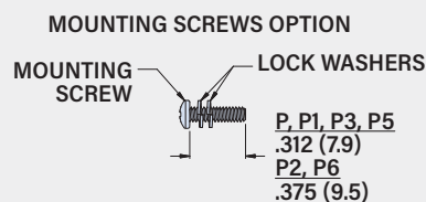
FIGURE 1 MOUNTING SCREWS
