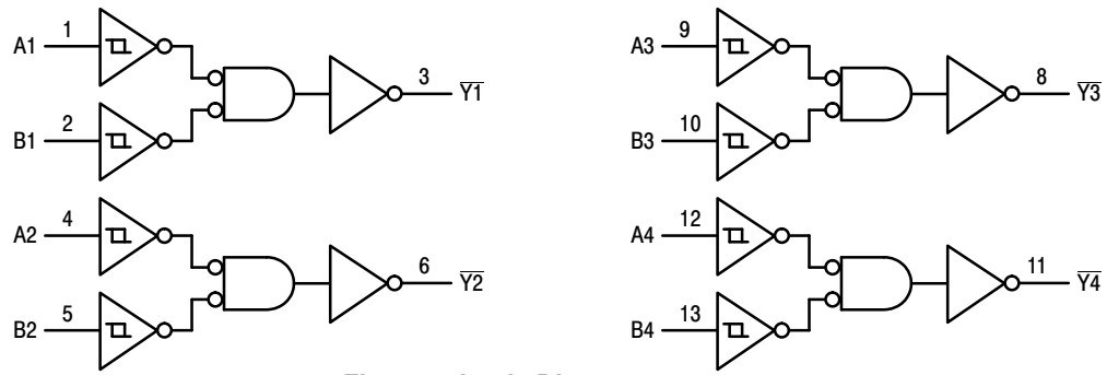
Figure 2. Logic Diagram
