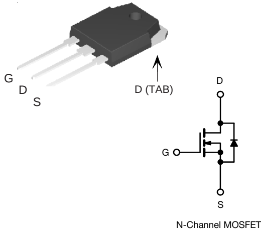
N-Channel MOSFET
