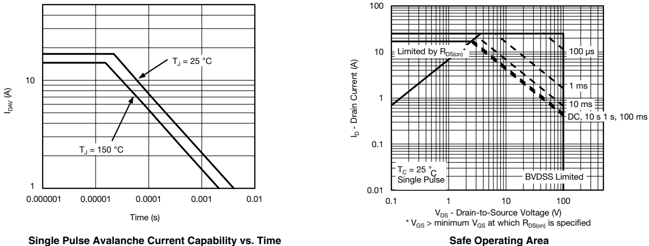
Single Pulse Avalanche Current Capability vs. Time
