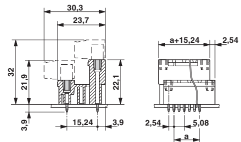
Dimensional drawing
