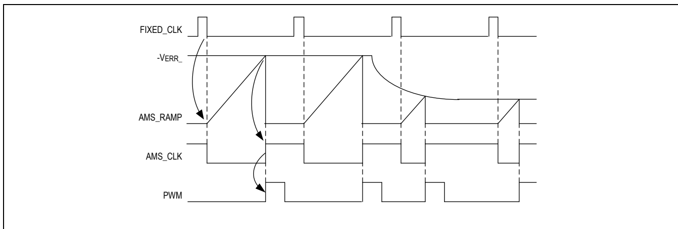
Figure 2. AMS Operation
