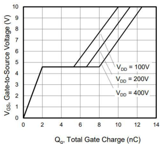
Figure 8. Gate Charge
