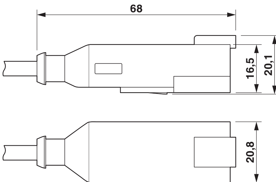
DEUTSCH DT04-4P, top view and side view
