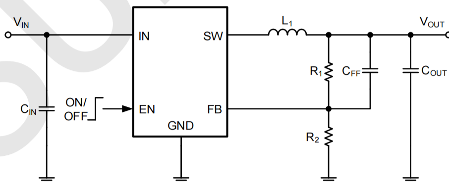
Basic Application Circuit
