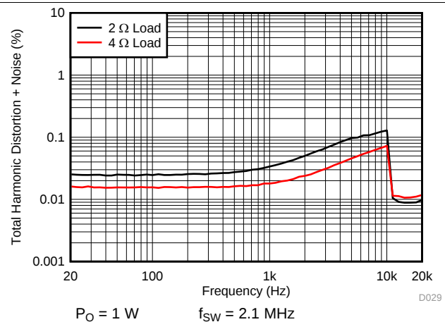
Figure 12. PBTLD THD+N vs Frequency
