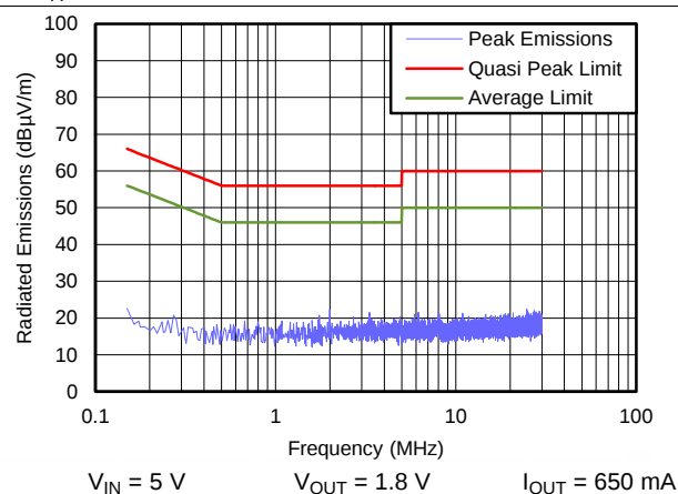
Figure 8. Conducted EMI Default Evaluation Board BOM With Additional 2.2μh 1μf LC Input Filter
