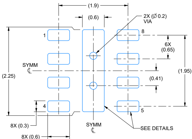
LAND PATTERN EXAMPLE 1:1 RATIO WITH PACKAGE SOLDER PADS SCALE: 20X
