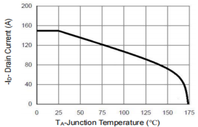
Figure 10 Current De-rating
