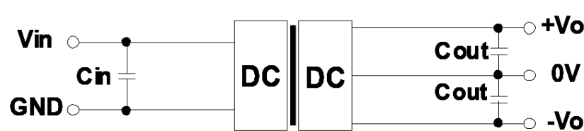
Figure 2 Dual Output Models
