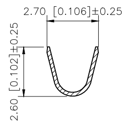
SECTION:A-A SCALE:1:1
