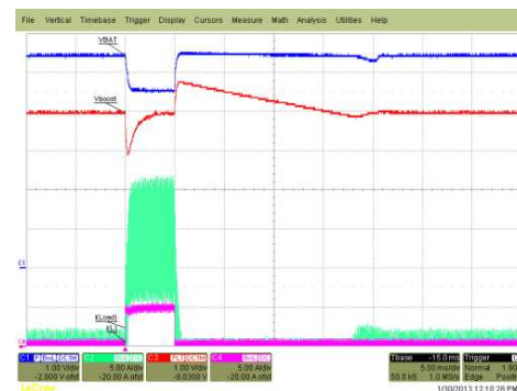
Figure 6. Load Step Response (Boost) (0 to 5 A at 10 A/ \mu\text{s} )
