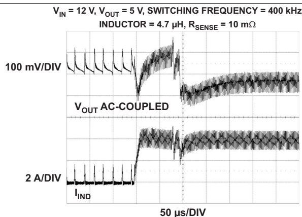
Figure 5. Buck Load Step: Low-Power-Mode Exit (90 mA to 4 A at 2.5 A/ \mu\text{s} )
