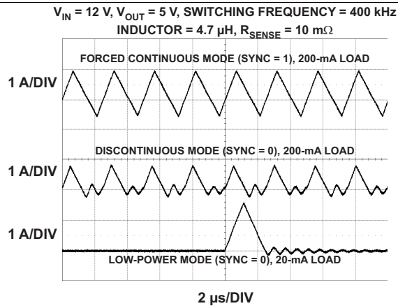
Figure 1. Inductor Currents (Buck)
