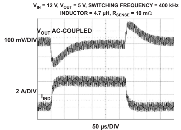
Figure 2. Buck Load Step: Forced Continuous Mode (0 to 4 A at 2.5 A/ \mu\text{s} )
