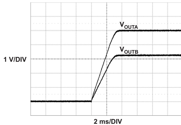
Figure 3. Soft-Start Outputs (Buck)
