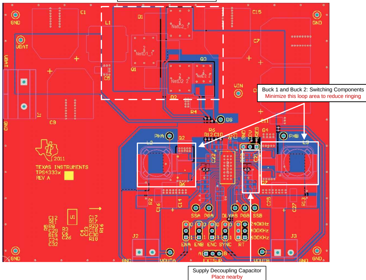
Figure 28. Layout Example (Top)
