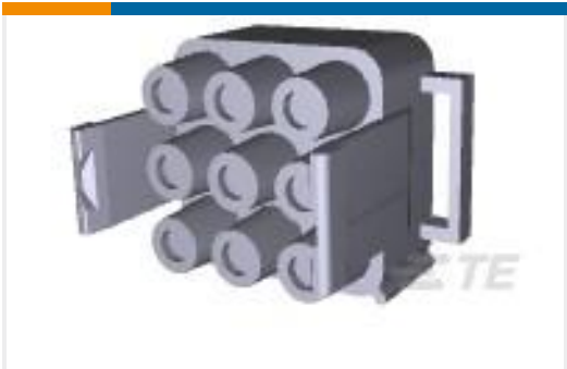
TE Part #770040-1 09P UMNL II PLUG REAR 94VO
