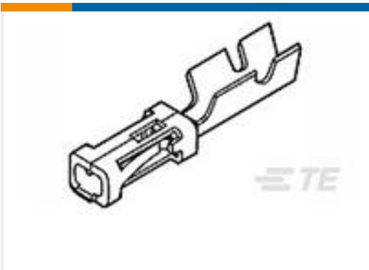
TE Part #87756-4 MOD IV RECP PLTD 15 SEL
