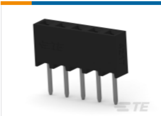
TE Part #2314876-5 5P,2MM,B-B,REC,SRVT,2,7,0.1AU,TB
