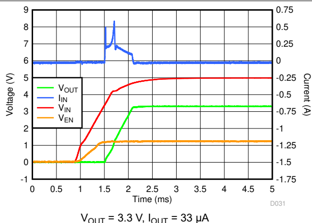
Figure 7-34. Startup Inrush Current With C_{OUT} = 47\text{ }\mu\text{F}
