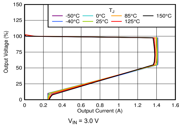
Figure 7-19. Foldback Current Limit vs Temperature
