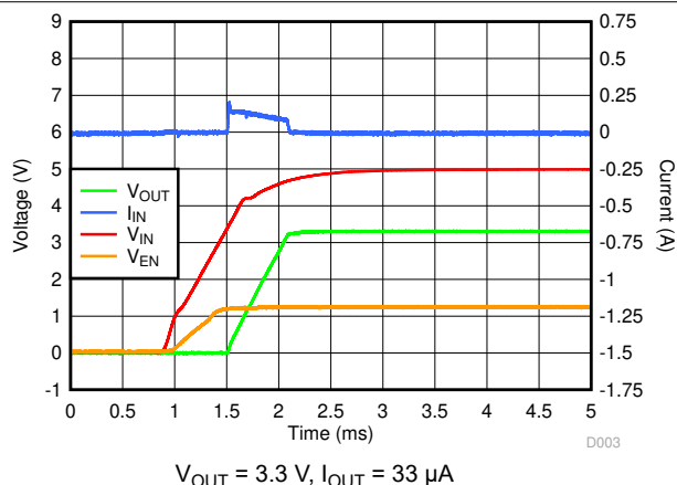
Figure 7-33. Startup Inrush Current With C_{OUT} = 22\text{ }\mu\text{F}
