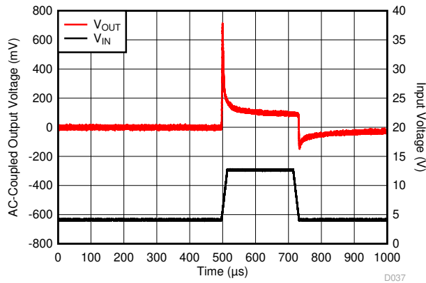
Figure 7-13. V_{IN} Transient in Dropout From 4 V to 13 V
