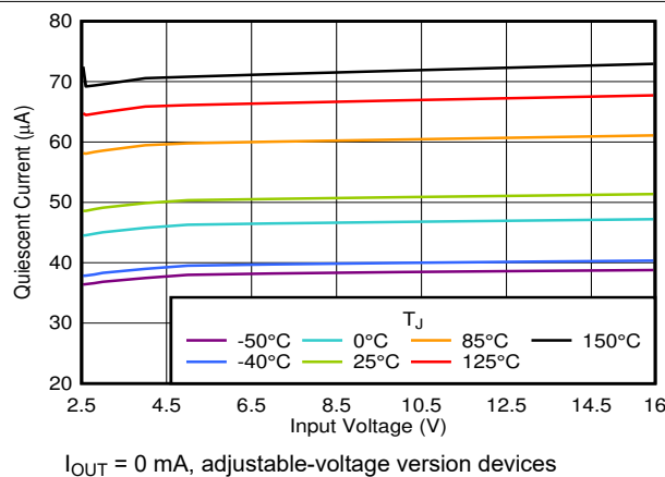
Figure 7-5. I_Q vs V_{IN}
