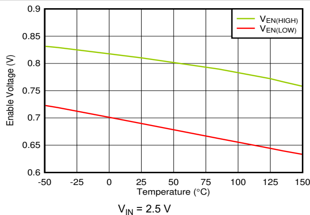
Figure 7-23. V_{EN} Thresholds vs Temperature
