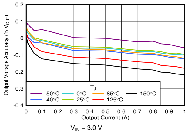
Figure 7-1. V_{OUT} Accuracy vs I_{OUT}
