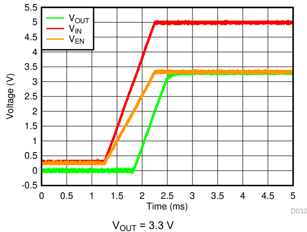
Figure 7-21. Startup With Separate V_{EN} and V_{IN}
