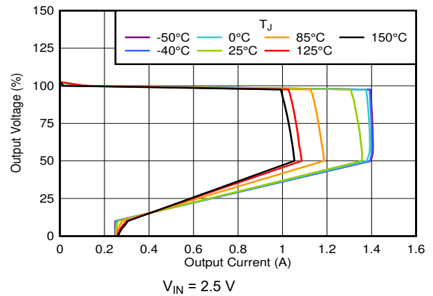
Figure 7-20. Foldback Current Limit vs Temperature
