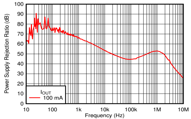
Figure 9-4. PSRR Performance
