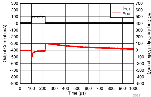
Figure 9-3. Load Transient Response, I_{OUT} 0 mA to 100 mA
