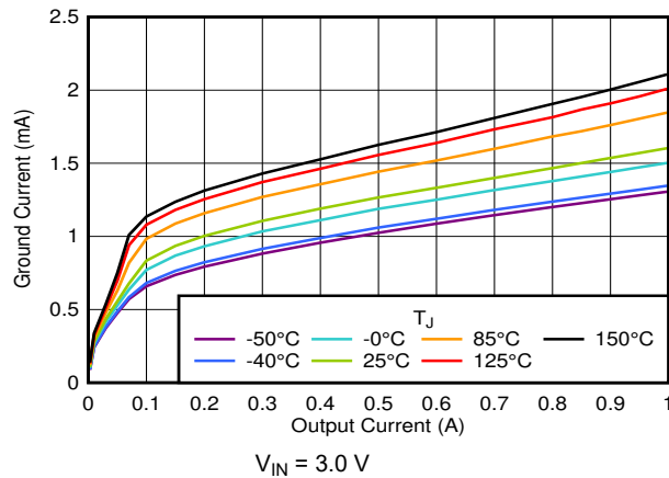
Figure 7-7. I_{GND} vs I_{OUT}
