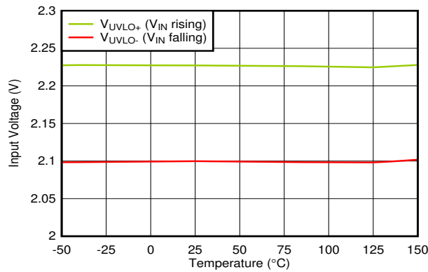
Figure 7-25. UVLO Thresholds vs Temperature
