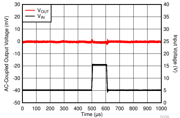
Figure 7-14. V_{IN} Transient From 5 V to 16 V
