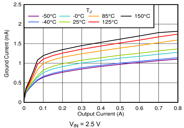
Figure 7-8. I_{GND} vs I_{OUT}
