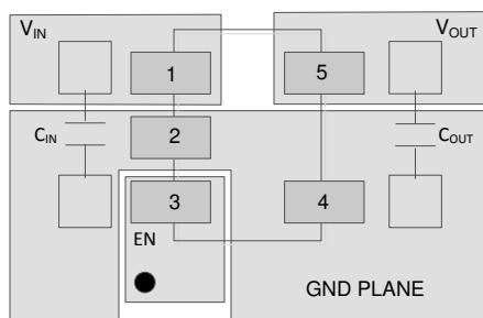
Figure 11-3. Layout Example for the Fixed HVSSOP Version
