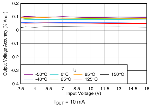
Figure 7-3. V_{OUT} Accuracy vs V_{IN}
