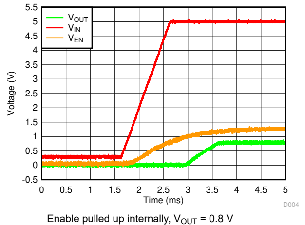
Figure 7-22. Startup With V_{EN} Floating
