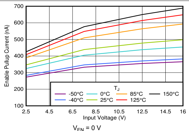
Figure 7-30. I_{EN} vs V_{IN}
