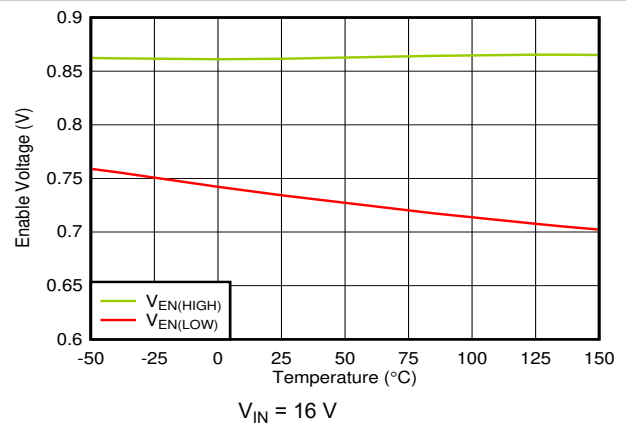
Figure 7-24. V_{EN} Thresholds vs Temperature
