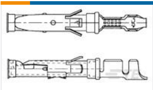
TE Part #163087-9 062 SOC.ASS. TYP3+
