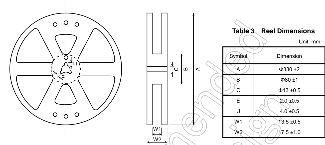
Figure 4 Reel Form
