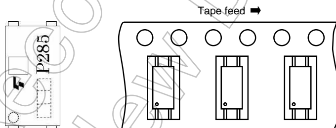
Figure 2 Device Orientation
