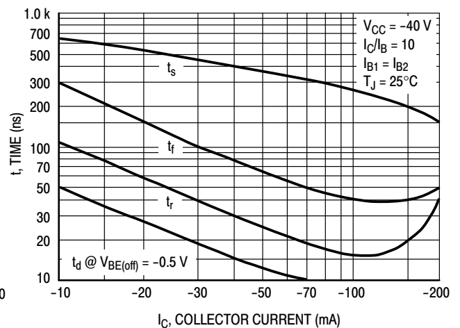
Figure 8. Switching Times
