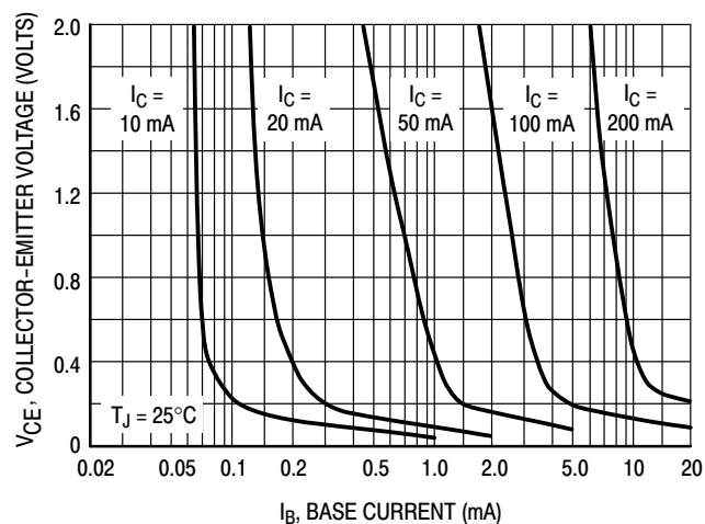
Figure 16. Collector Saturation Region
