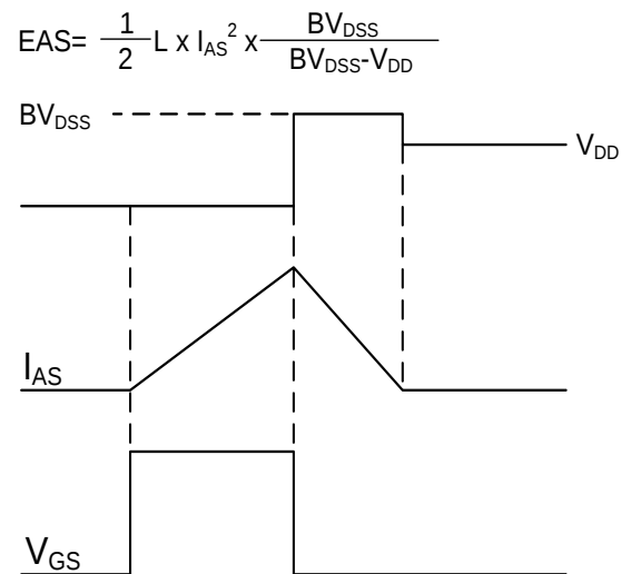
Fig.8 EAS Waveform
