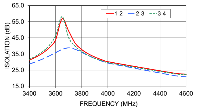
WP4S+ ISOLATION
