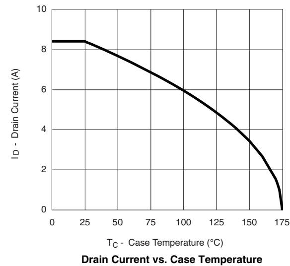
Drain Current vs. Case Temperature
