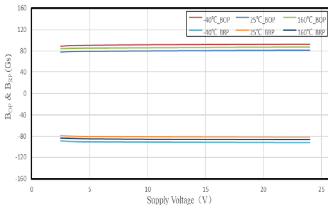
SC2448 B_{OP} & B_{RP} VS. Supply Voltage
