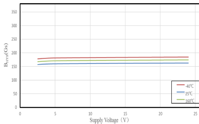
SC2448 B_{HYS} VS. Supply Voltage
