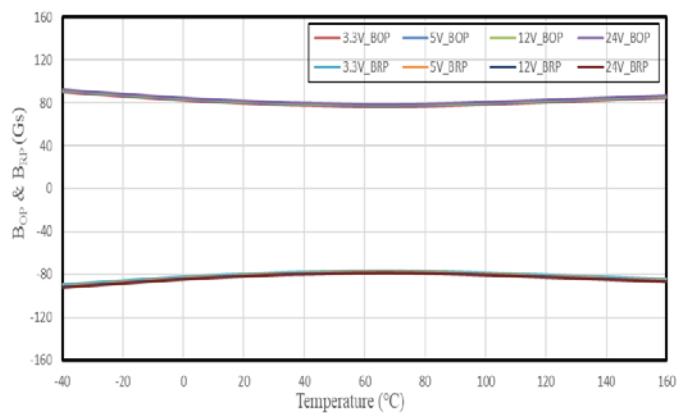
SC2448 B_{OP} & B_{RP} VS. Temperature
