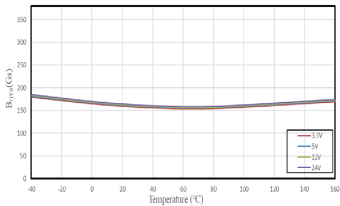
SC2448 B_{HYS} VS. Temperature
