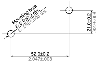
Mounting dimensions
