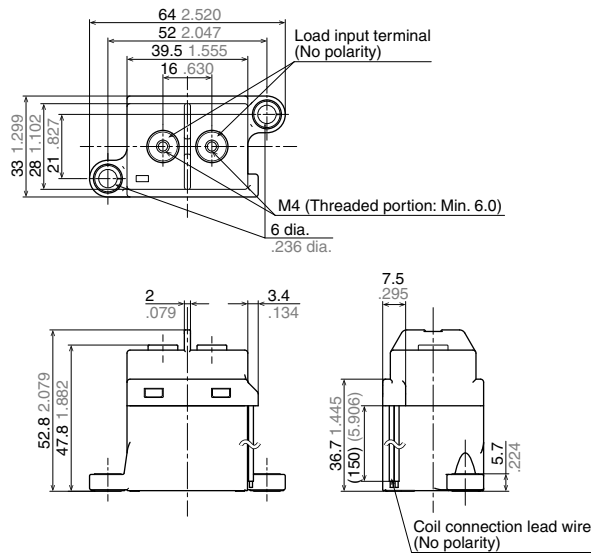
External dimensions
