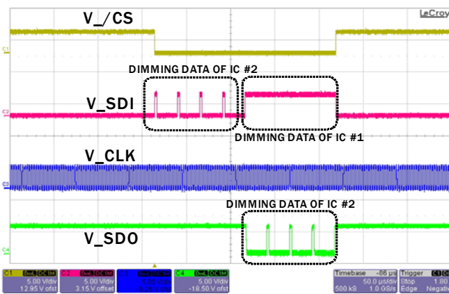
FIGURE 14. TIMING OF SPI INTERFACE (TWO ICs DAISY CHAINED, CS : 120Hz, CLK : 390kHz, f_{DIM} : 200Hz)
