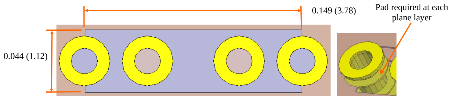
Figure 20: Option 1 Elongated Rectangular Backplane Antipad Clearance.
