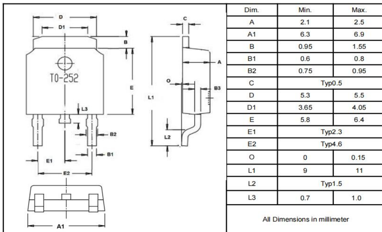
TO-252
