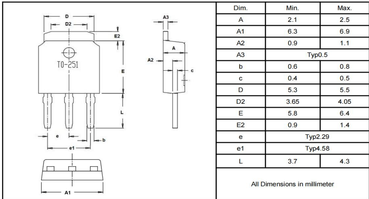
TO-251
