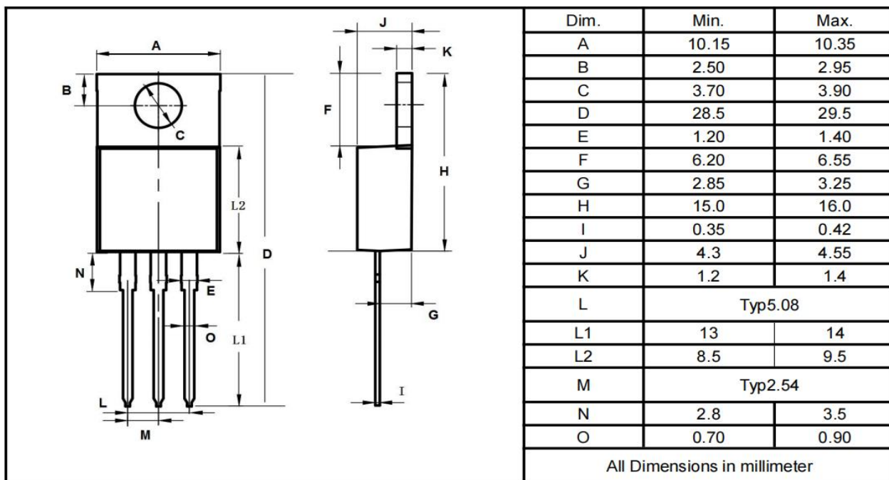
TO-220AB
