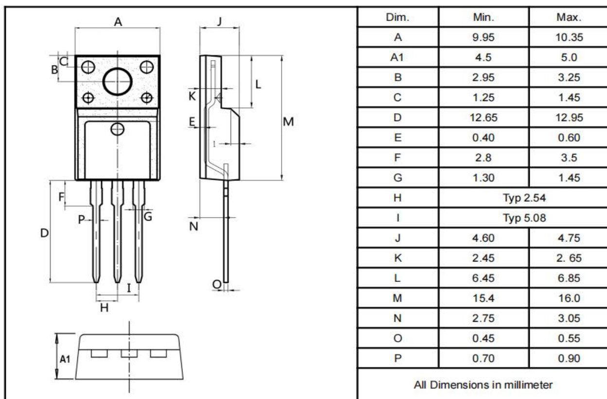
TO-220F
