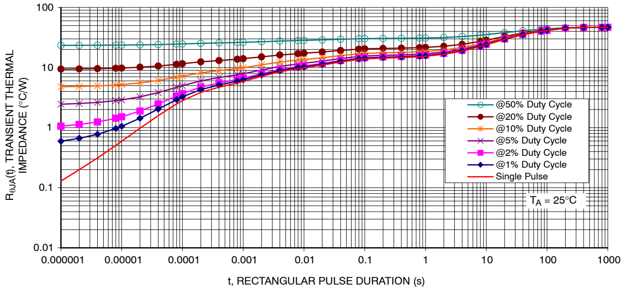
Figure 13. Thermal Response
