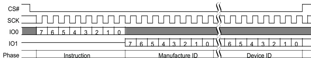
Figure 9-1 READ_ID (90h) Command Sequence
