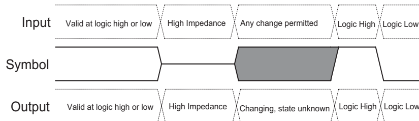
Figure 5-1 Waveform Element Meanings
