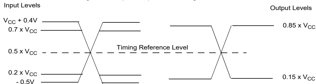
Figure 5-2 Input, Output, and Timing Reference Levels
