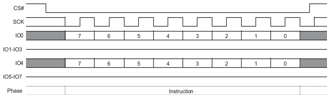
Figure 9-51 Dual-Quad Software Reset (RESET F0h) Command Sequence
