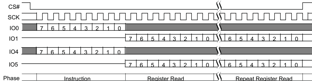
Figure 9-8 Read Bank Register (BRRD 16h) Command
