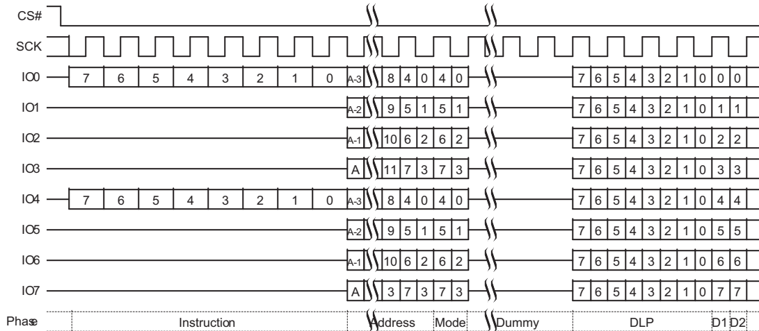
Figure 9-28 Dual-Quad SPI DDR Quad I/O Read Initial Access
