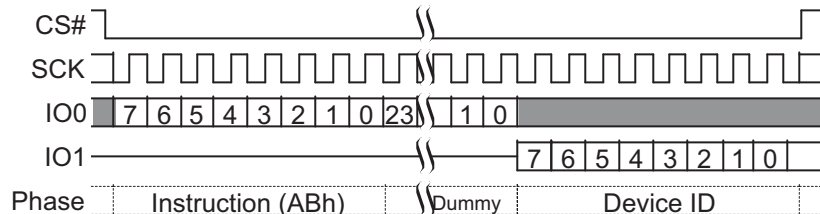
Figure 9-3 Read Electronic Signature (RES ABh) Command Sequence
