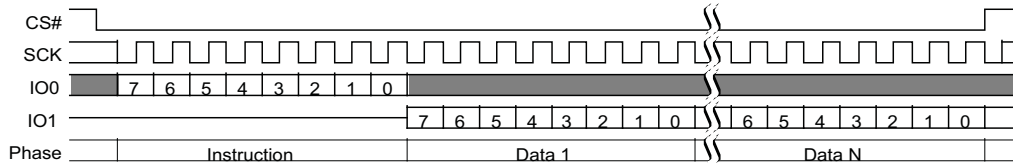
Figure 9-2 Read Identification (RDID 9Fh) Command Sequence
