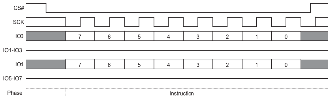
Figure 9-52 Dual-Quad SPI Mode Bit (MBR FFh) Reset Command Sequence
