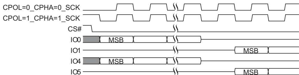
Figure 3-1 Dual-Quad SPI SDR Modes Supported
