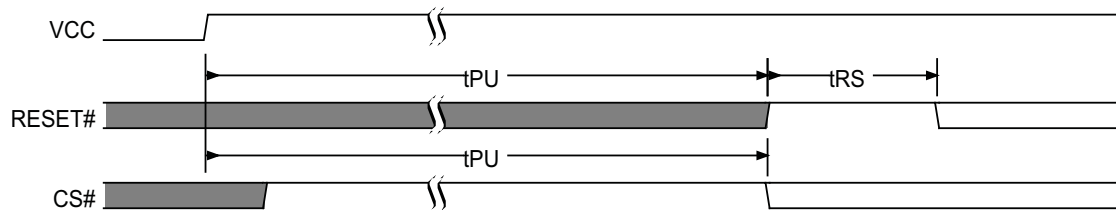
Figure 5-6 POR followed by Hardware Reset
