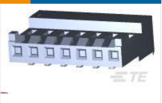
TE Part #3-643817-7 07P MTA156 CONN ASSY 18AWG ORA
