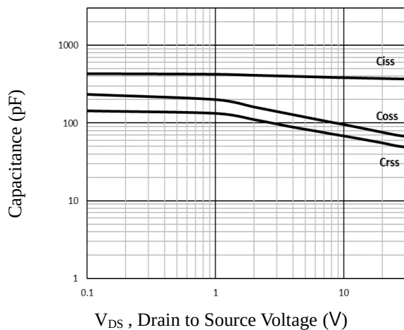
Fig.7 Capacitance Characteristics
