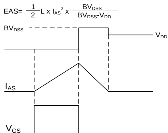
Fig.11 EAS Waveform
