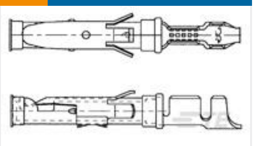
TE Part #163091-8 062 SOC.ASS. TYP3+
