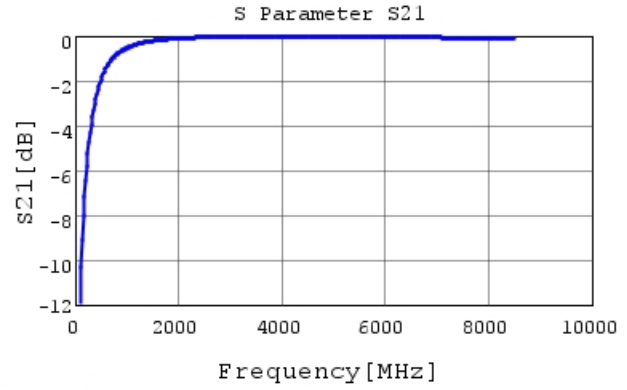
GJM1555C1H4R2BB01 S21 DCOV, 25degC
