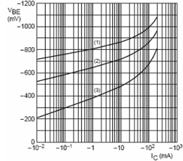
BC857A; V_{CE} = -5\text{ V} . (1) T_{amb} = -55\text{ }^{\circ}\text{C} . (2) T_{amb} = 25\text{ }^{\circ}\text{C} . (3) T_{amb} = 150\text{ }^{\circ}\text{C} .
