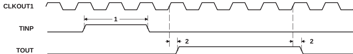
Figure 38. Timer Timing
