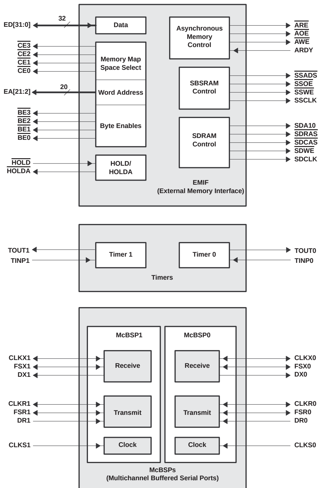
Figure 3. Peripheral Signals
