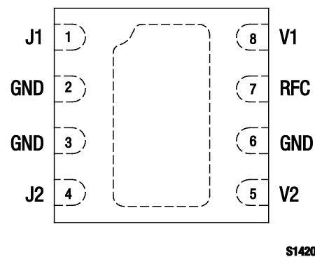
Figure 2. SKY13321-360LF Pinout – 8-Pin QFN (Top View)
