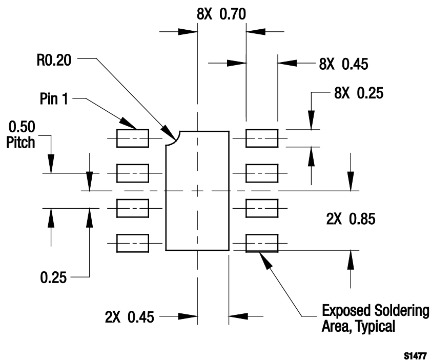
Figure 10. SKY13321-360LF PCB Layout Footprint
