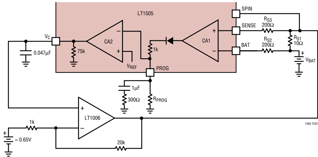
Test Circuit 2
