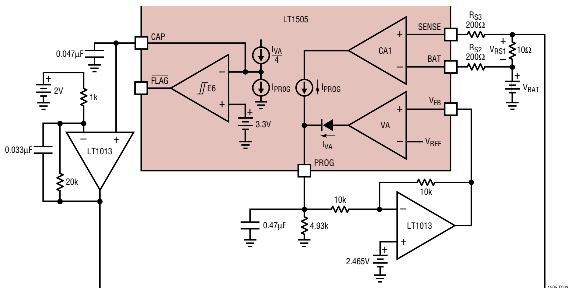
Test Circuit 3
